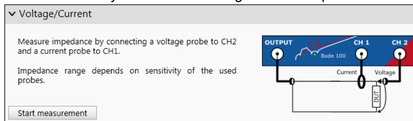
Figure 6: Voltage/Current measurement mode
